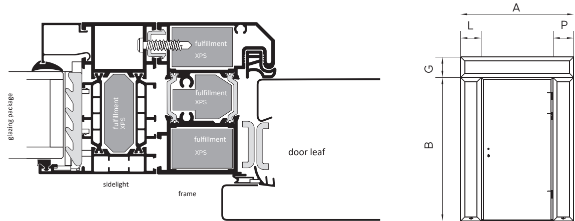
Comfort 73 door with side light
